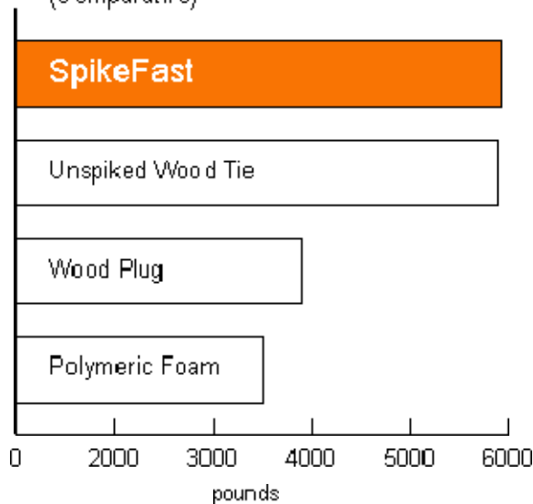
Spike Withdrawal Force Results (Comparative)
