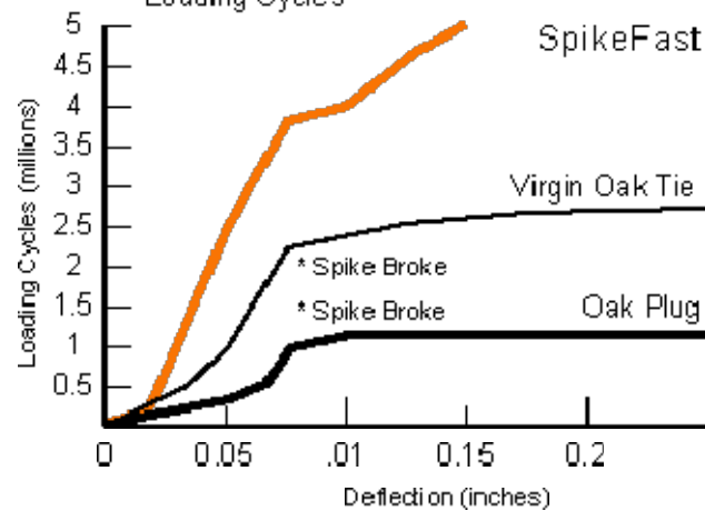
Spike Deflection vs. Dynamic Loading Cycles
